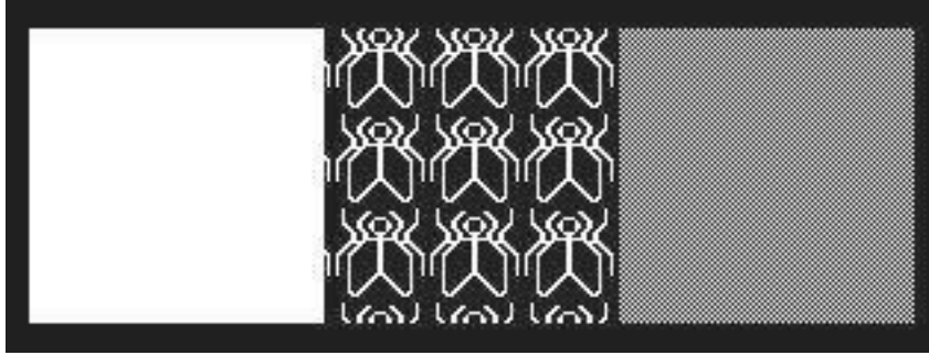
Figure 2-11 Stippled Polygons
