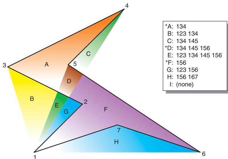
Figure 14-2 Concave Polygon
