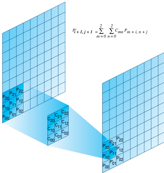
Figure 8-15 The Pixel Convolution Operation
