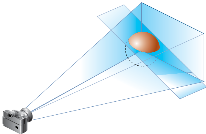
Figure 3-22 Additional Clipping Planes and the Viewing Volume
