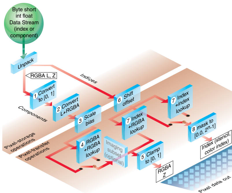
Figure 8-12 Drawing Pixels with glDrawPixels()
