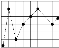
Figure 3-16 Viewport Rectangle
