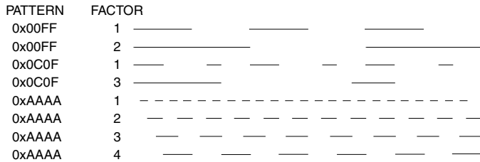
Figure 2-8 Stippled Lines
