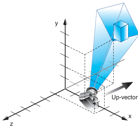
Figure 3-12 Using gluLookAt()
