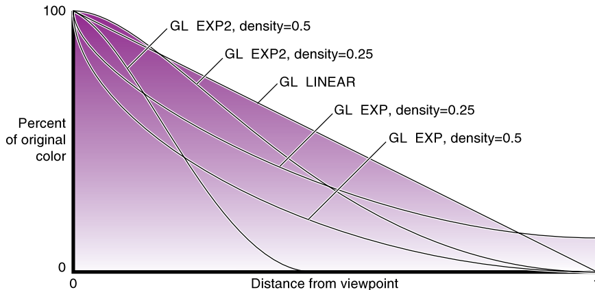
Figure 6-4 Fog-Density Equations
