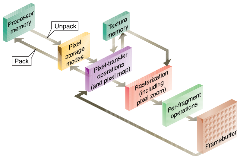
Figure 8-5 Imaging Pipeline
