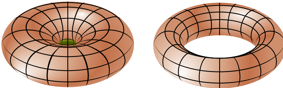
Figure 9-9 Texture-Map Distortion
