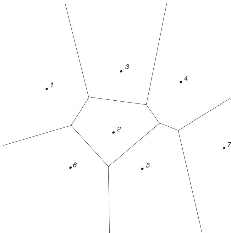
Figure 14-3 Dirichlet Domains
