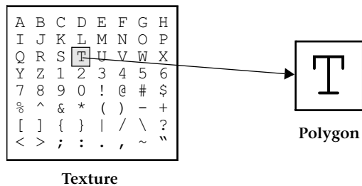
Figure 9-7 Using a Mosaic Texture
