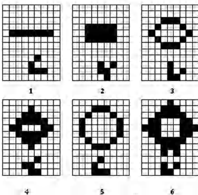
Figure 14-4 Six Generations from the Game of Life
